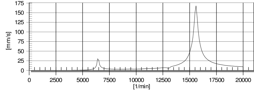
Unbalance response
