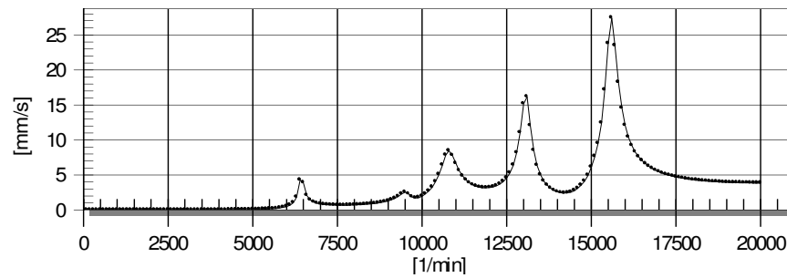
Unbalance response
