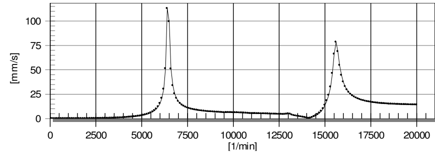
Unbalance response
